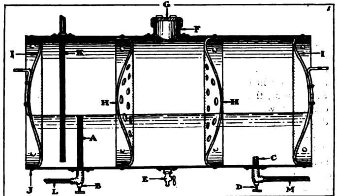
Fig. 1.—Partitioned gasoline tank entrapping a reserve supply.
